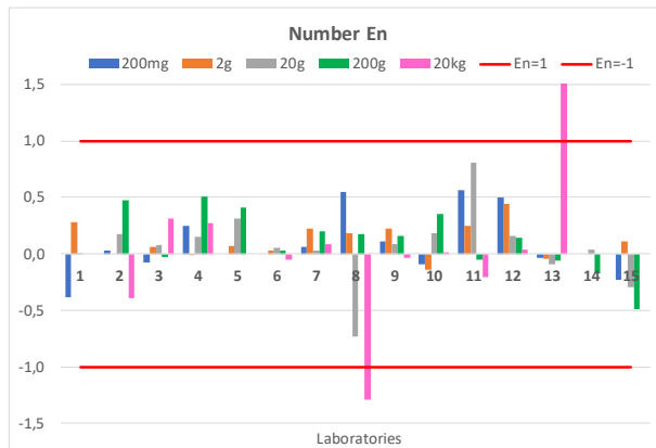
Fig. 8. Numbers En for all the masses
