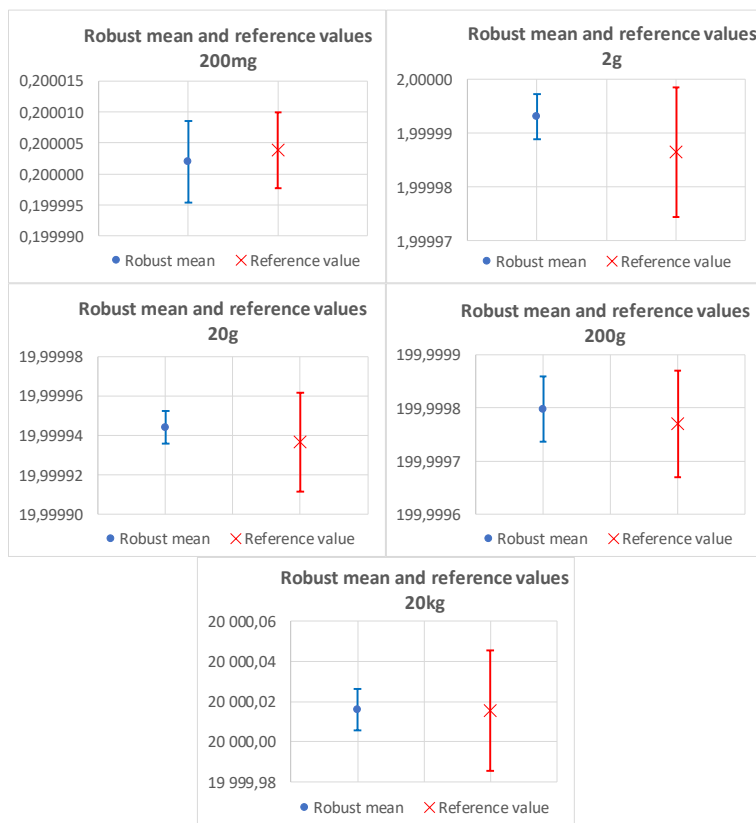
Fig. 1. Comparison between the robust means and the reference values
