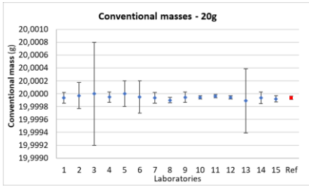
Fig. 4a. Conventional masses and their uncertainties for 20g
