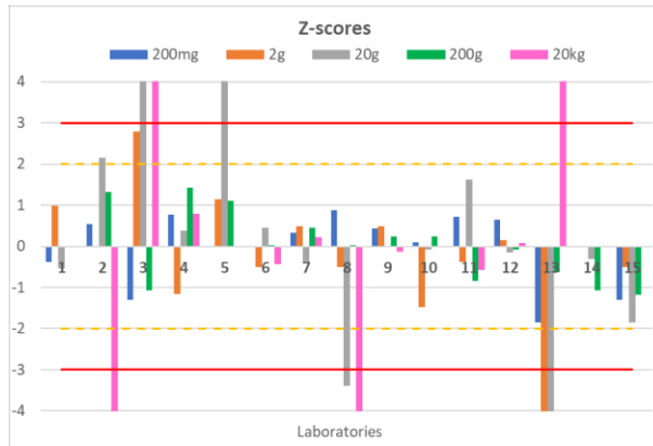
Fig. 7. Z-scores of each participant for all the calibrated masses
