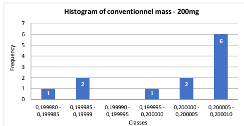
Fig. 2b. Histogram of conventional mass for 200mg
