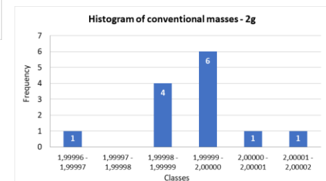
Fig. 3b. Histogram of conventional masses for 2g
