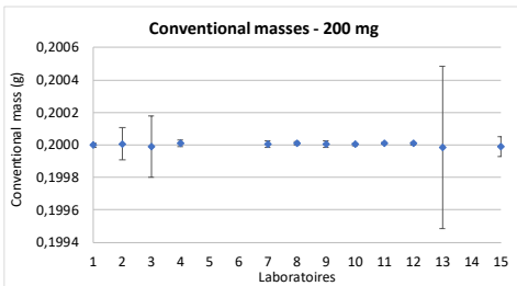
Fig. 2a. Conventional masses and their uncertainties for 200mg
