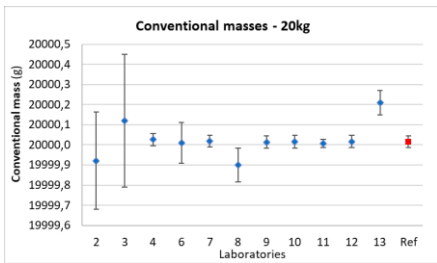
Fig. 6a. Conventional masses and their uncertainties for 20kg
