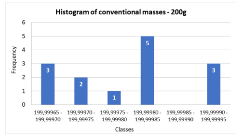
Fig. 5b. Histogram of conventional masses for 200g
