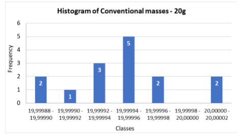
Fig. 4b. Histogram of conventional masses for 20g
