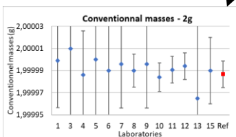
Fig. 3a. Conventional masses and their uncertainties for 2g
