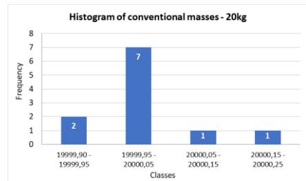
Fig. 6b. Histogram of conventional masses for 20kg
