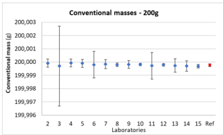
Fig. 5a. Conventional masses and their uncertainties for 200g
