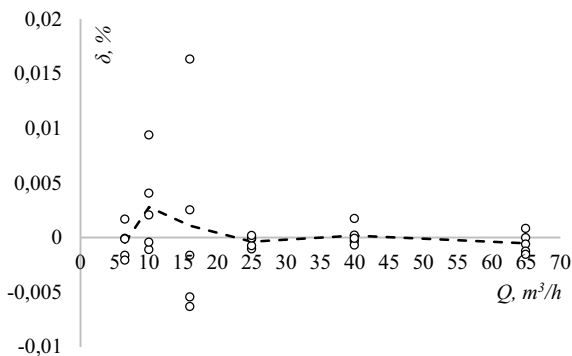
Figure 6. Additional error \delta_{\Delta P} as function of volumetric flowrate Q
