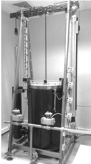
Figure 3. Combined bell-type prover. General view
