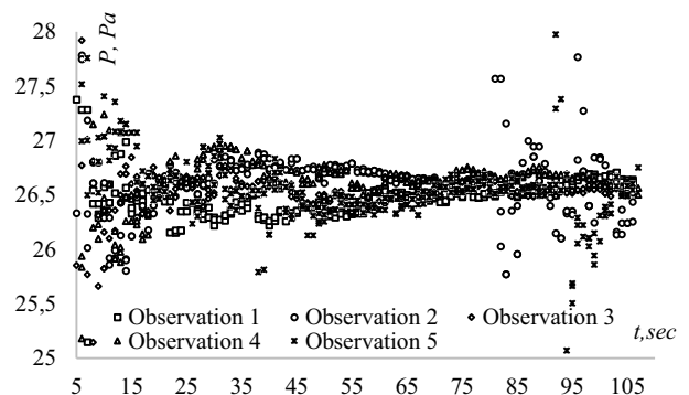
Figure 5. Pressure distribution for five independent observations at volumetric flowrate Q=10 m 3 /h
