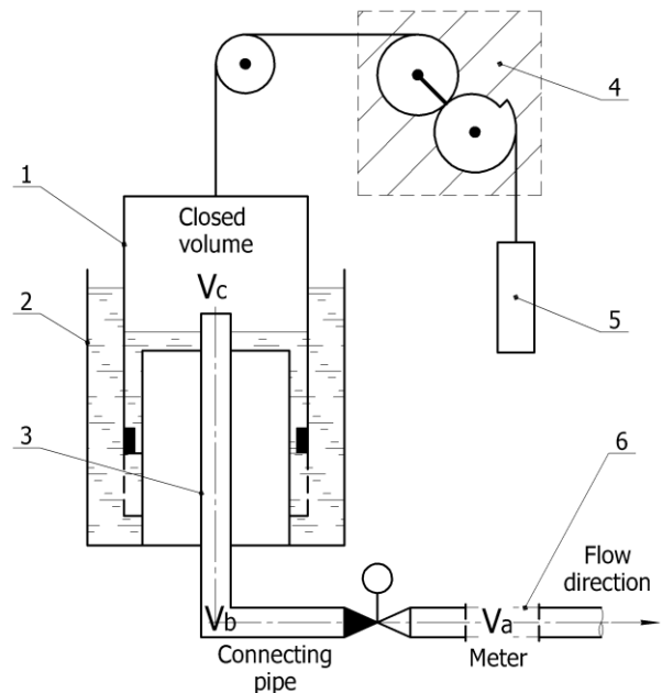
Figure 1. Standard bell-type prover principle scheme
