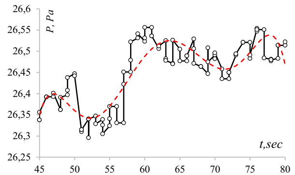
Figure 4. Pressure dependence under the bell P(\nu) and its approximation at Q=10 m 3 /h, \bar{\nu}=7,511 \cdot 10^{-3} m/sec
