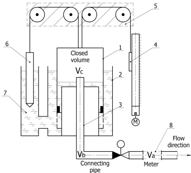
Figure 2. Combined bell-type prover. Principle scheme
