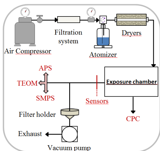
Fig. 1. Scheme of the experimental device
