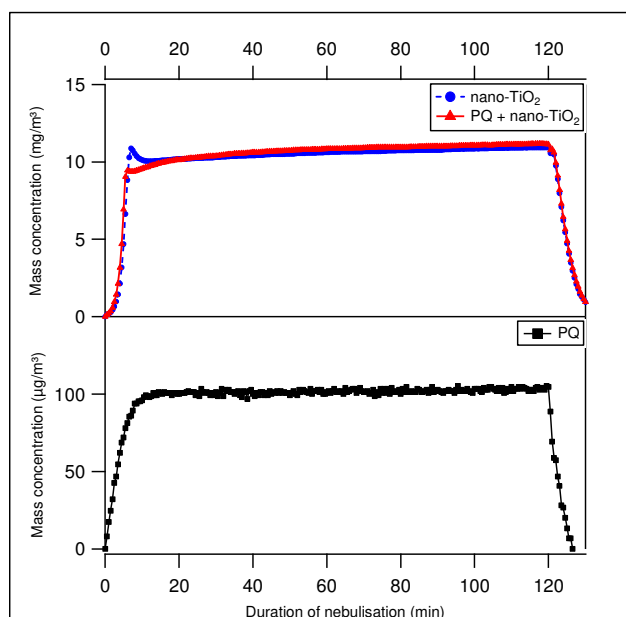
Fig. 2. Real-time total mass concentrations measurements for 120 min of experimentation.
