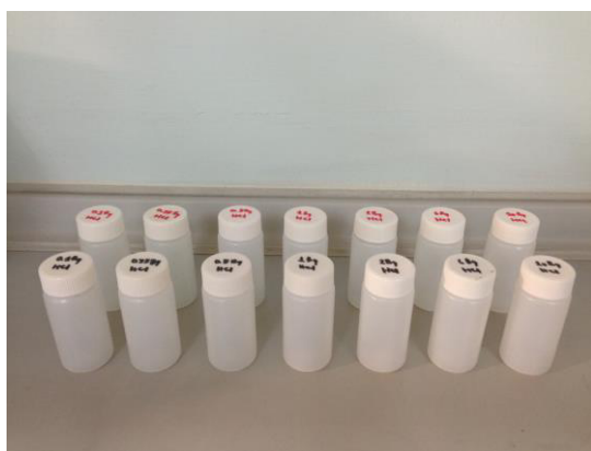
Figure 2. Series of ^{90}\text{Sr}/^{90}\text{Y} prepared solution sources of the 16 mL of 0.1 M HCl and 1 M \text{HNO}_3 in polyethylene vials.
